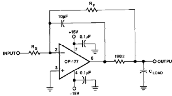
Figure 10. Isolating Capacitive Loads
